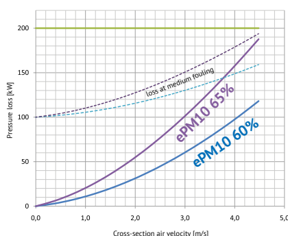
ePM10 60% and ePM10 65% Bag Filter Initial Pressure Loss
