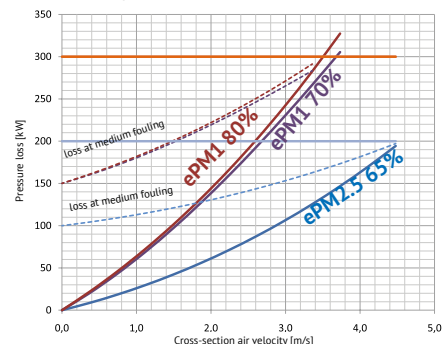
ePM2.5 65%, ePM1 70% and ePM1 80% Bag Filter Initial Pressure Loss
