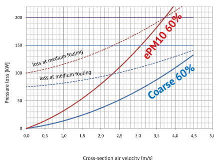
Frame Filter Insert Initial Pressure Loss
