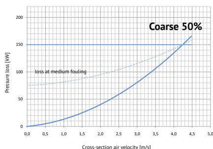
Woven Filter Insert Initial Pressure Loss
