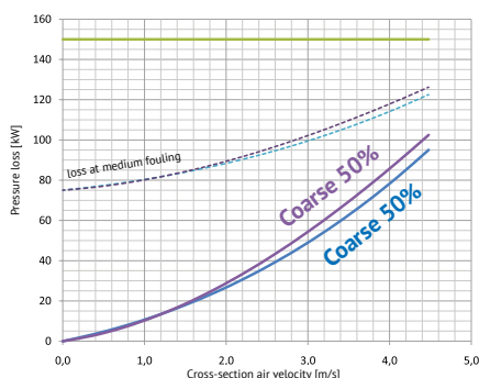
Coarse 50% and Coarse 60% Bag Filter Initial Pressure Loss
