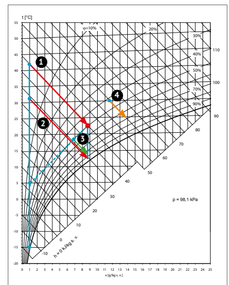
■ Honeycomb adiabatic humidifier
