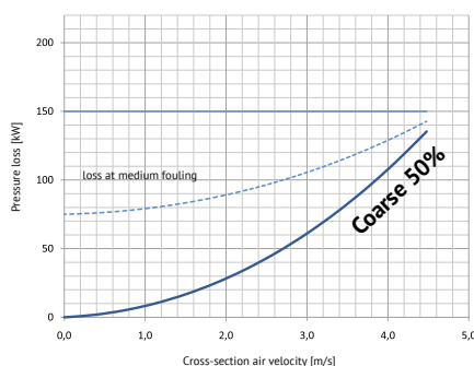
Metal Filter Initial Pressure Loss
