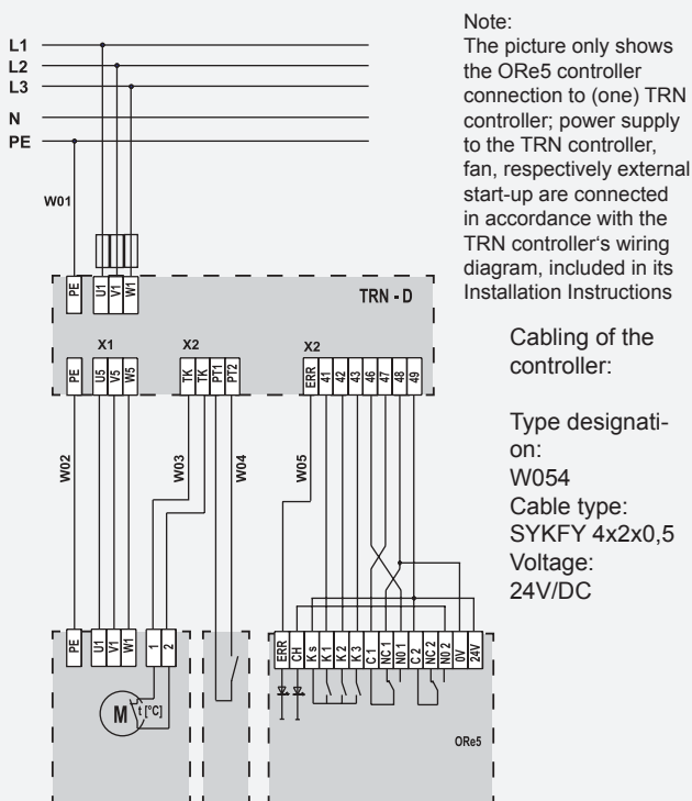
Figure 3 – Connection of the controller
