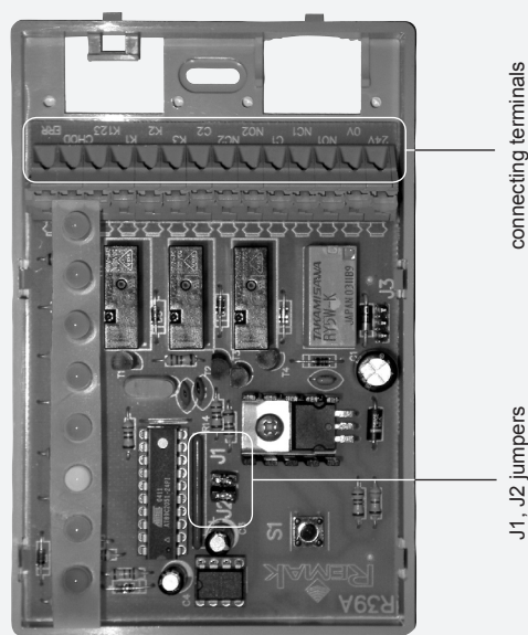
Figure 3 - Connection of the controller
