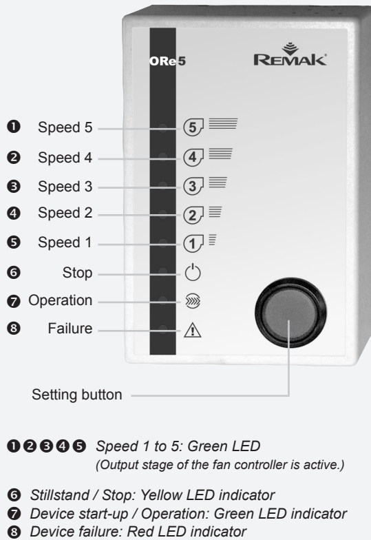
Figure 1 – Front panel and signalling
