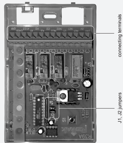
Figure 2 – Connection of the controller
